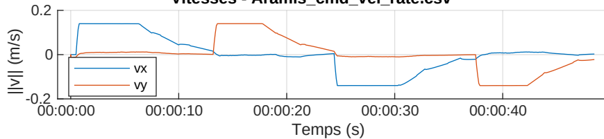
Vitesses - Aramis_cmd_vel_rate.csv
